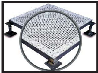
3M™ 8400 Series ESD Floor Tile is available in the special 24.5" x 24.5" size used for raised access floor panels.
